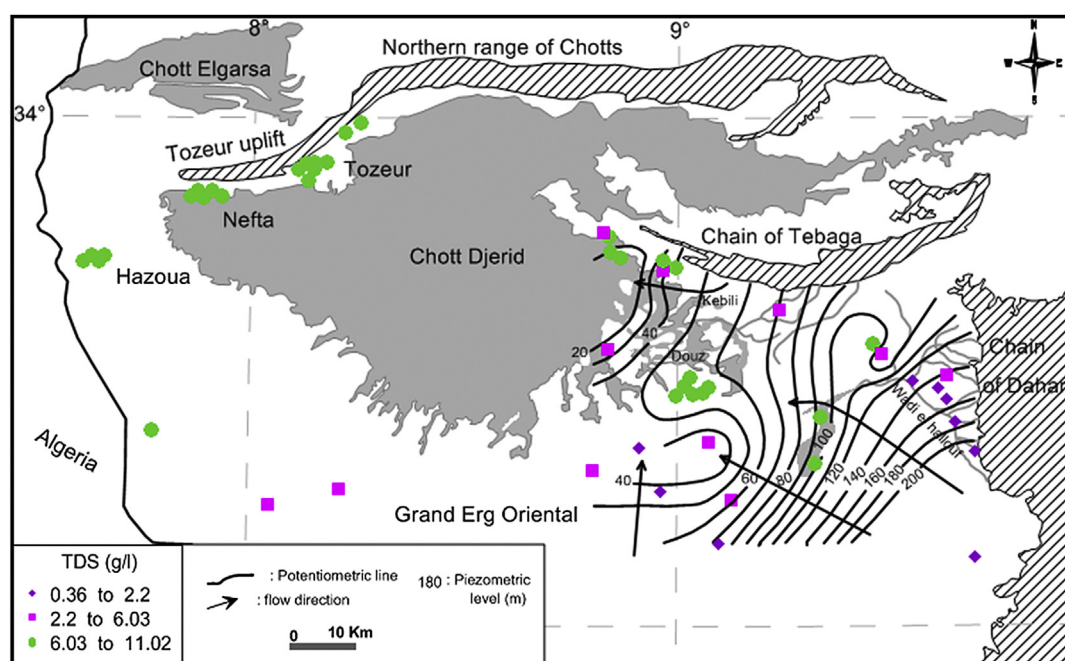
Fig. 2. Piezometric and salinity map of shallow aquifers in the studied area.
