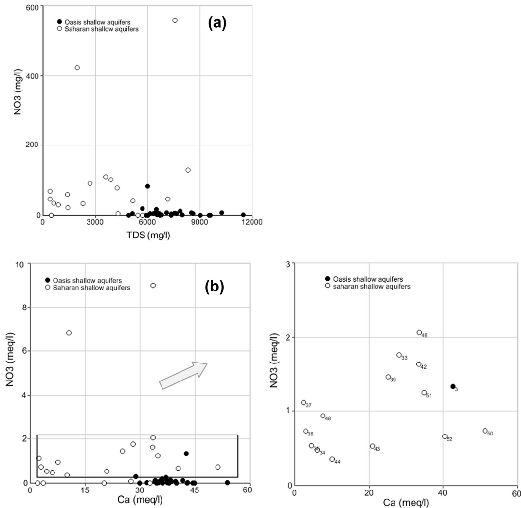
Fig. 11. TDS vs. \text{NO}_3^- (a) and \text{NO}_3^- vs. \text{Ca}^{2+} (b) relationships.
